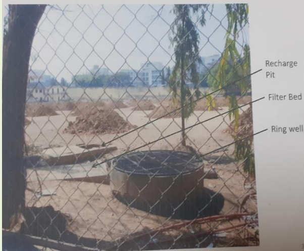
RING WELL, FILTER PIT, RECHARGE PIT
